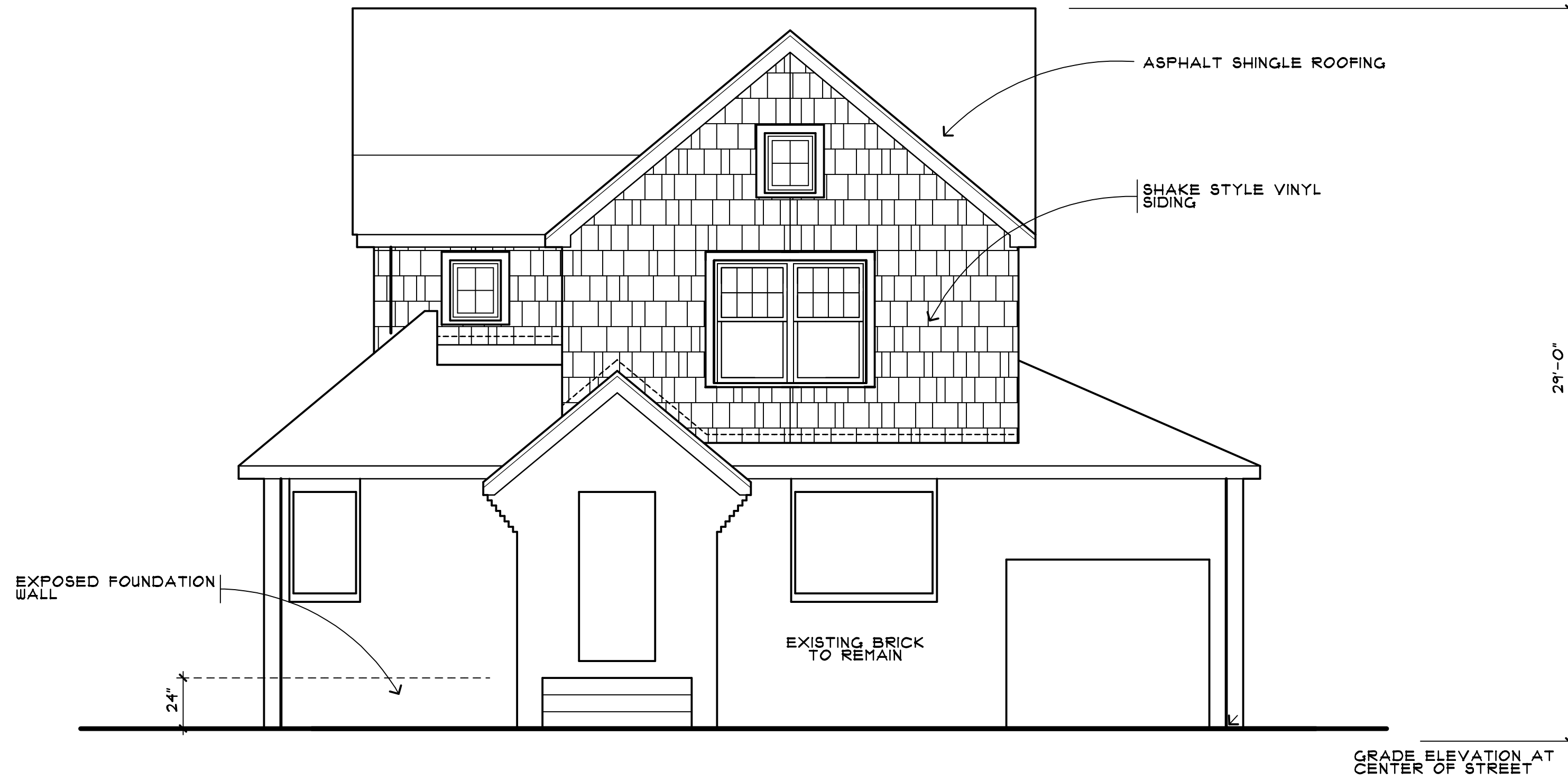
SOUTH ELEVATION
