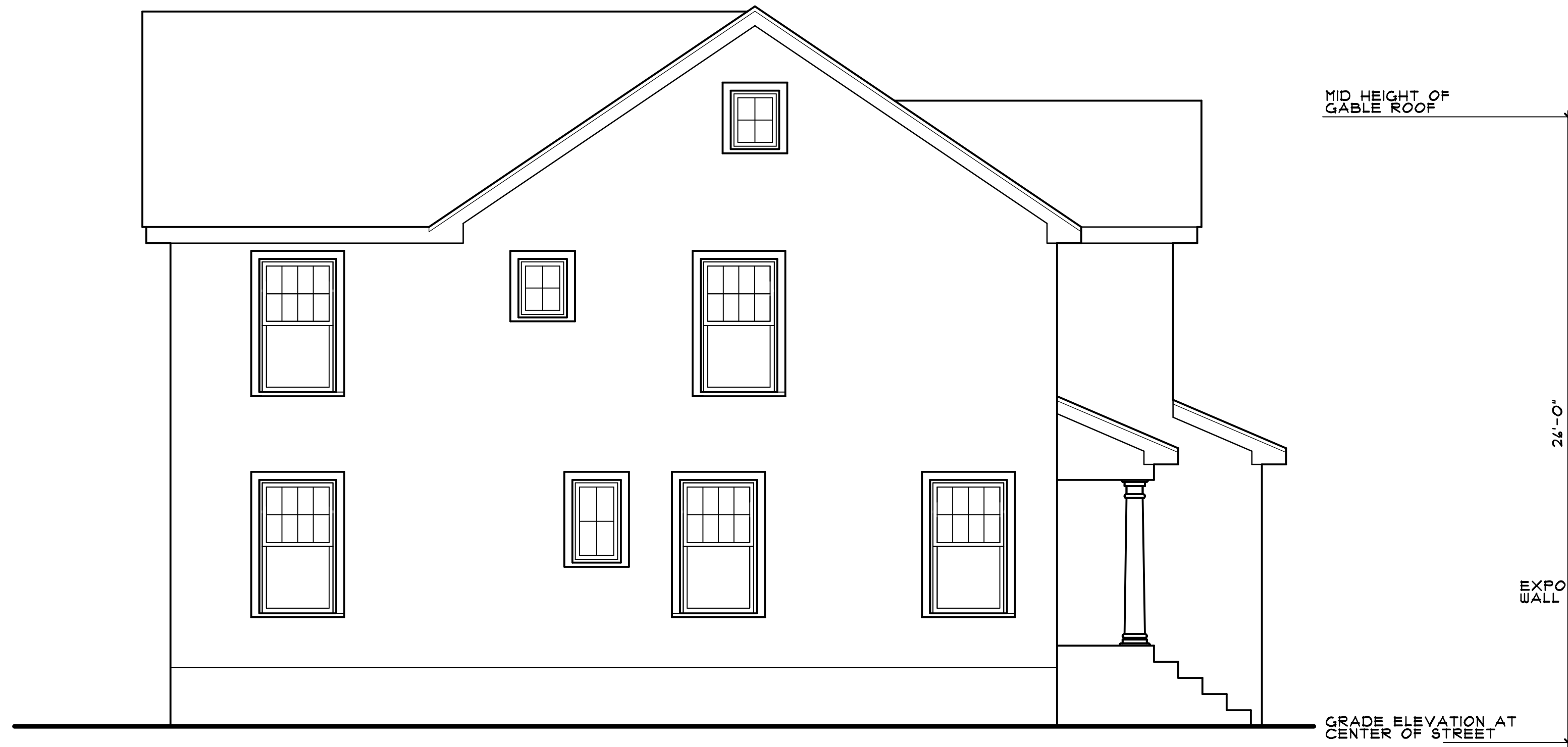
NORTH ELEVATION
