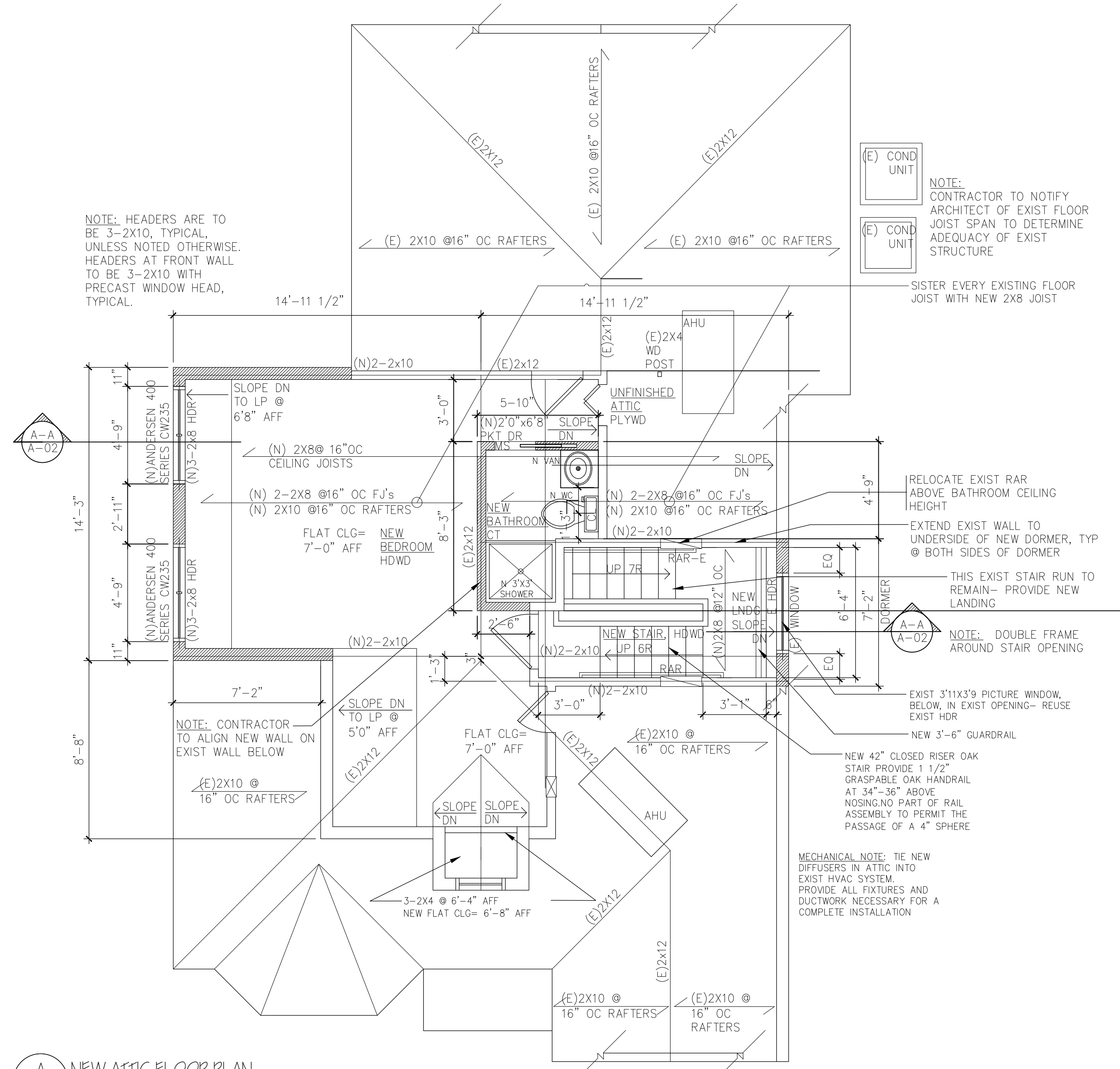
A NEW ATTIC FLOOR PLAN
