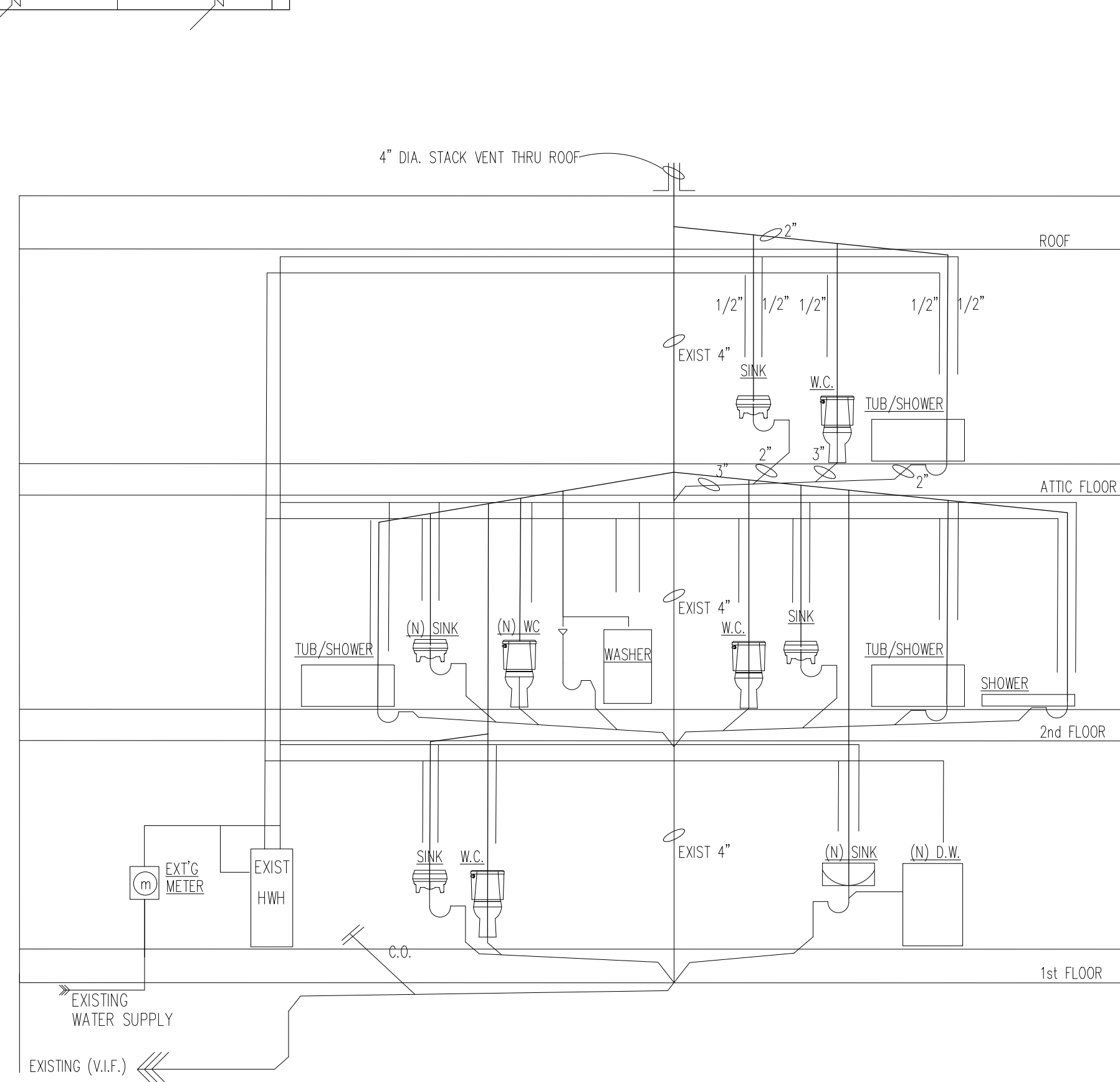
C PLUMBING RISER DIAGRAM
