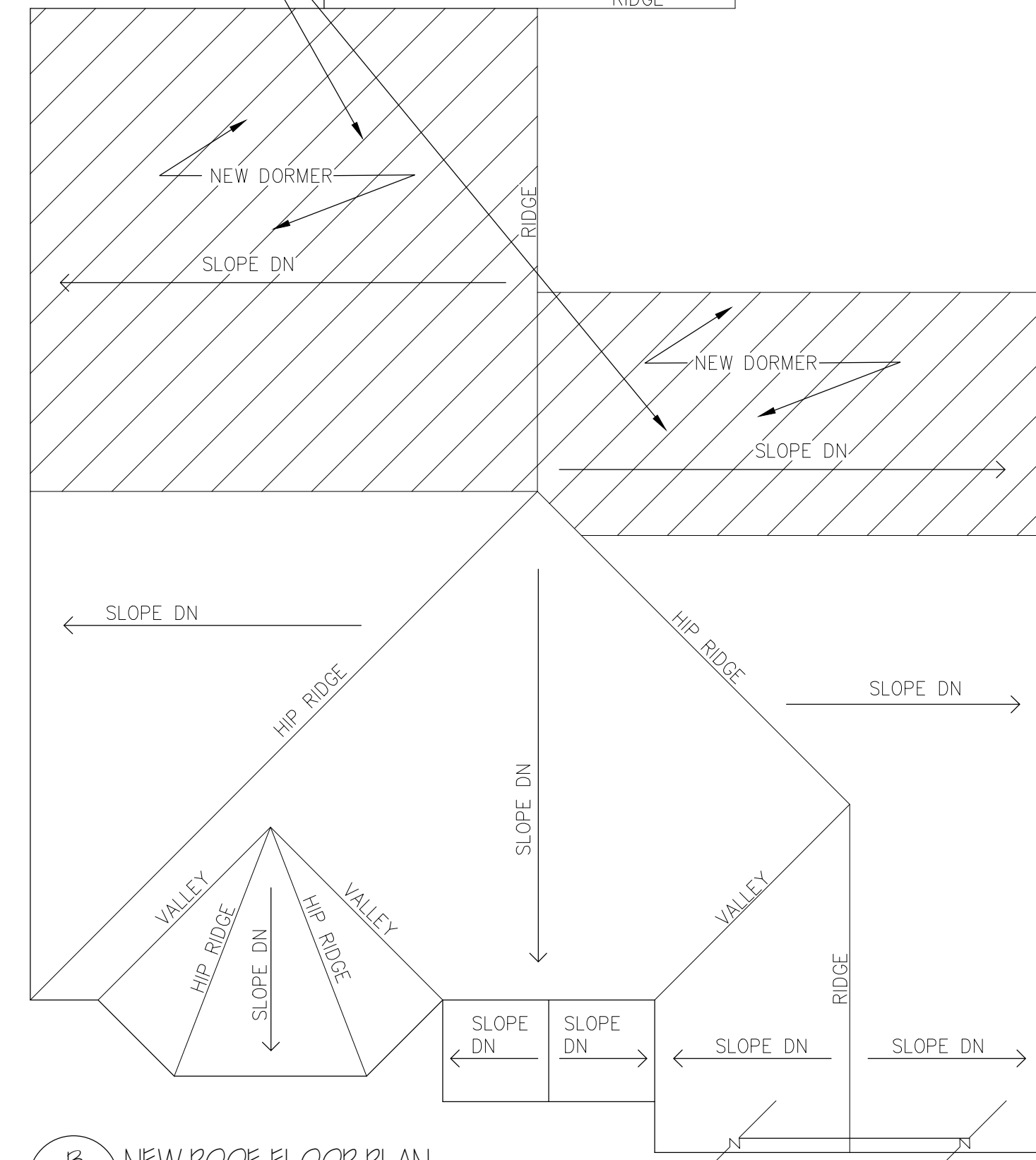
B NEW ROOF FLOOR PLAN
